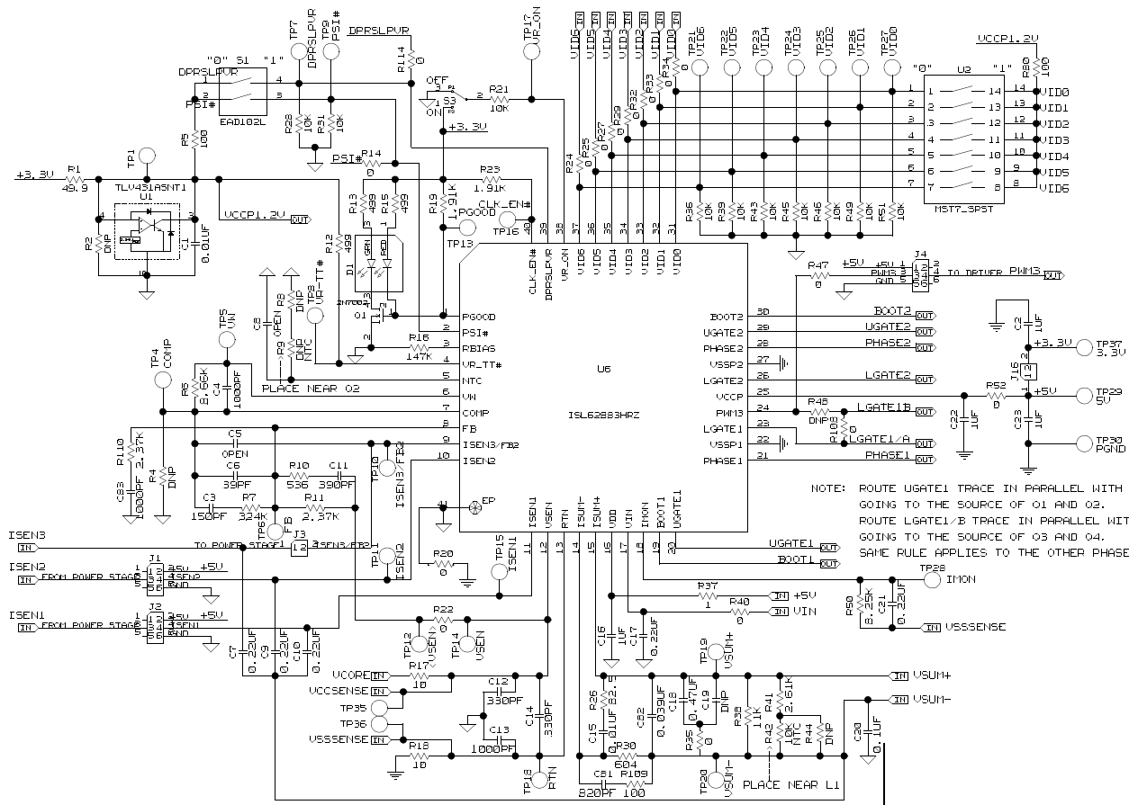
FIGURE 2. ISL62883EVAL2Z SCHEMATICS, PAGE 1 OF 5
