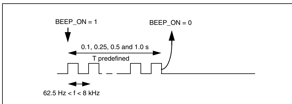
Figure 21: Pulse Mode
