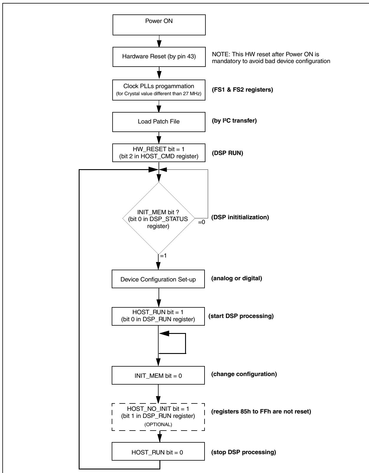
Figure 27: Flow chart
