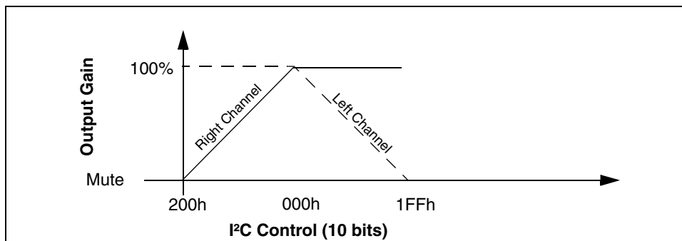
Figure 20: Differential Balance
