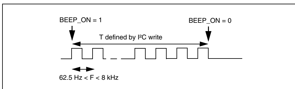
Figure 22: Continuous Mode
