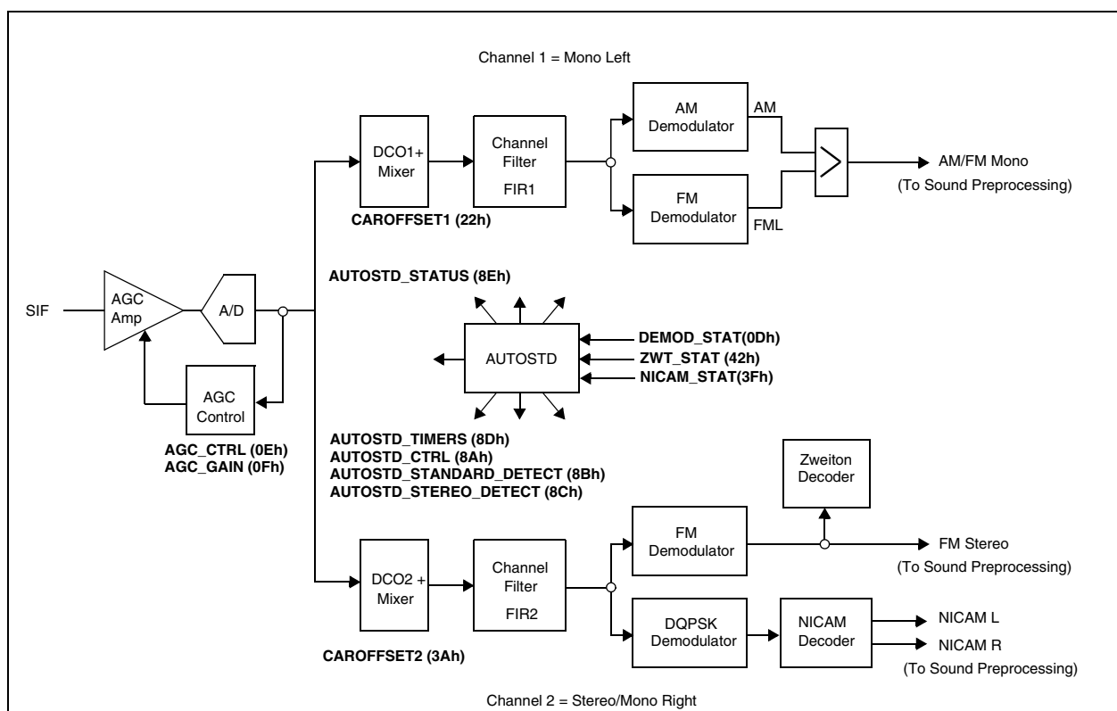
Figure 10: Demodulator Block Diagram
