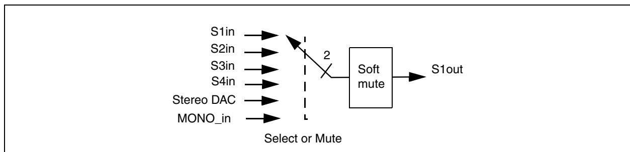
Figure 24: SCART1/2/3 Output Matrix
