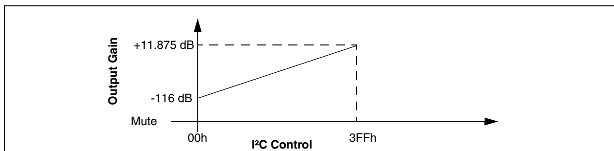
Figure 19: Volume Control
