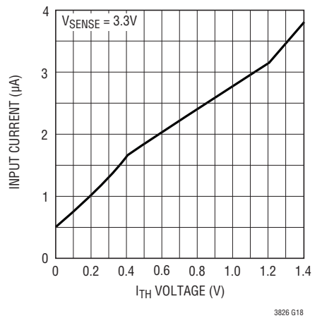
SENSE Pins Total Input Bias Current vs I TH
