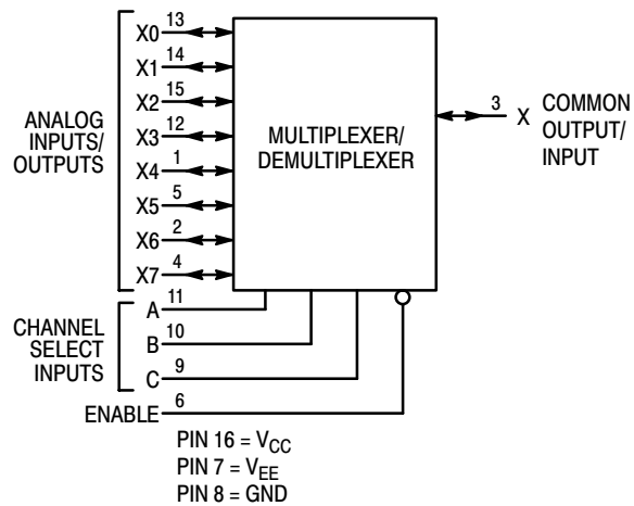
MC74VHC4051
