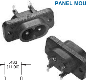
IEC-NC-A-4 RIGHT ANGLE PANEL MOUNT
