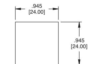
Recommended Panel Cut-Out For Panel 0.8mm - 1.50mm
