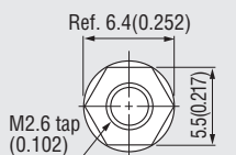
8850-SR-03 mounting panel t1.6mm(0.063)
