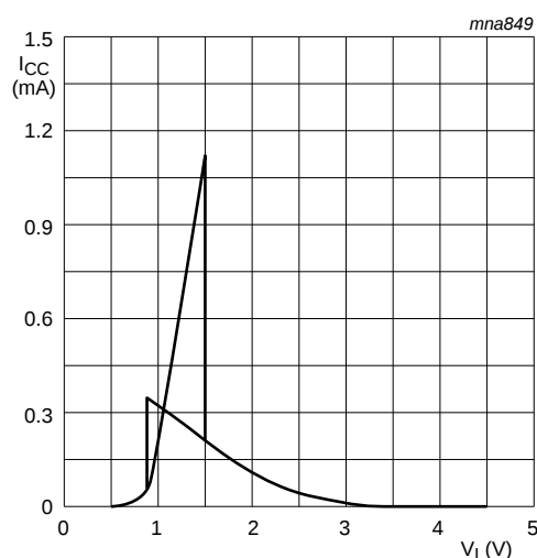
Fig 11. Typical 74HCT transfer characteristics
