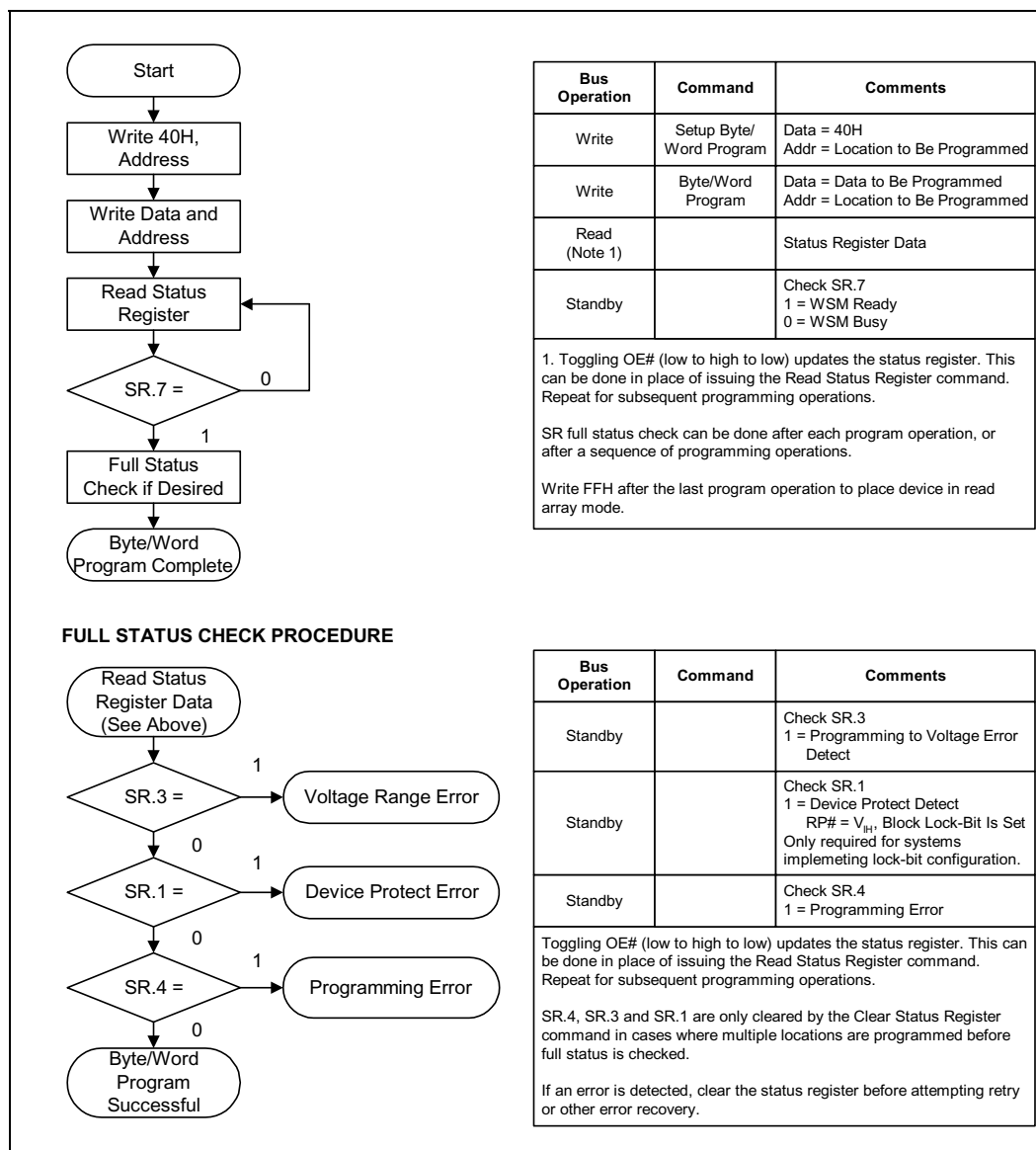
Figure 14. Byte/Word Program Flowchart
