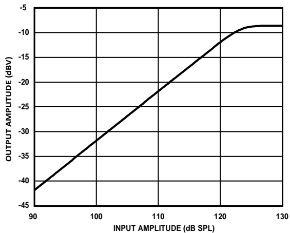
Figure 7. Linearity
