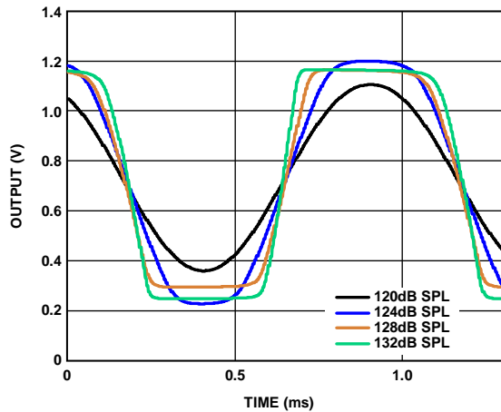
Figure 8. Clipping Characteristics
