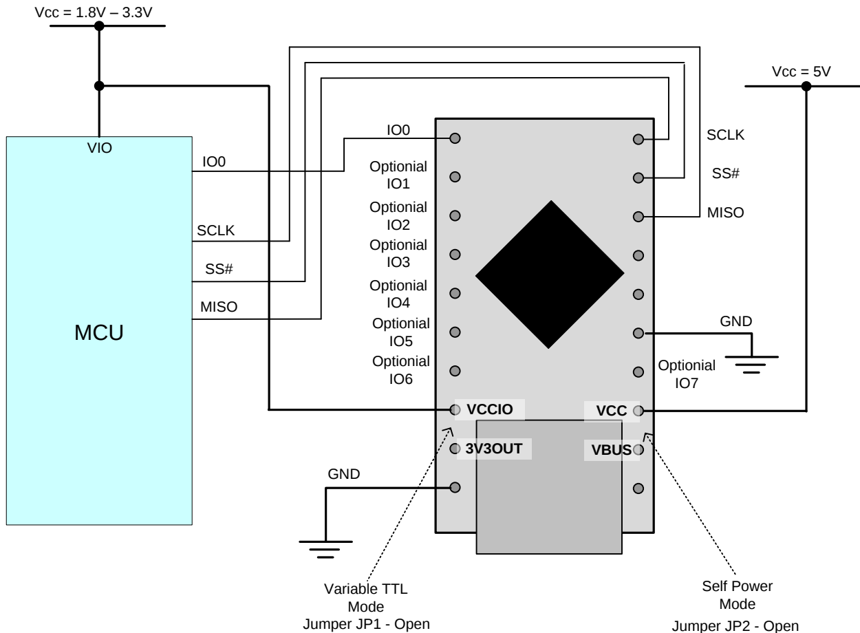
Figure 5.2 – Self-Powered Configuration
