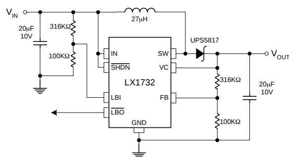
Figure 3 – V_{OUT} = 5.0V ; I_{OUT} = 150mA and V_{LBI} = 2.5V
