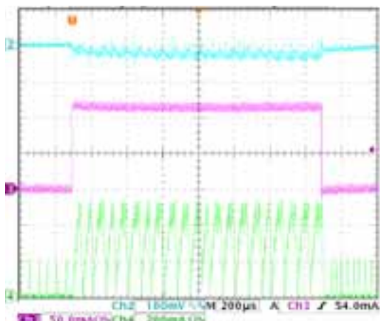
Figure 10: Step Load Response
