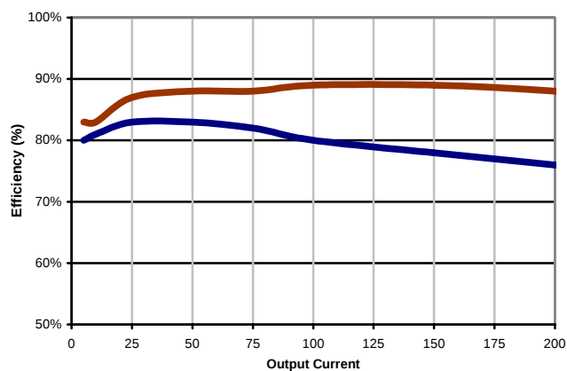
Figure 8 – Efficiency vs. Output Current (mA)
