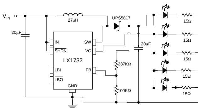
Figure 5 – LX1732 driving 5 white LEDs in parallel where V_{OUT} \geq 3.6V ; I_{OUT} = 100mA .
