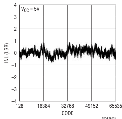
INL Curve
