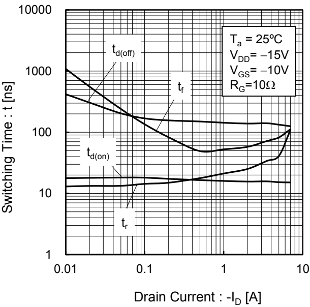
Fig.19 Switching Characteristics
