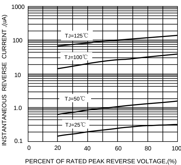
FIG.5-TYPICAL REVERSE CHARACTERISTICS
