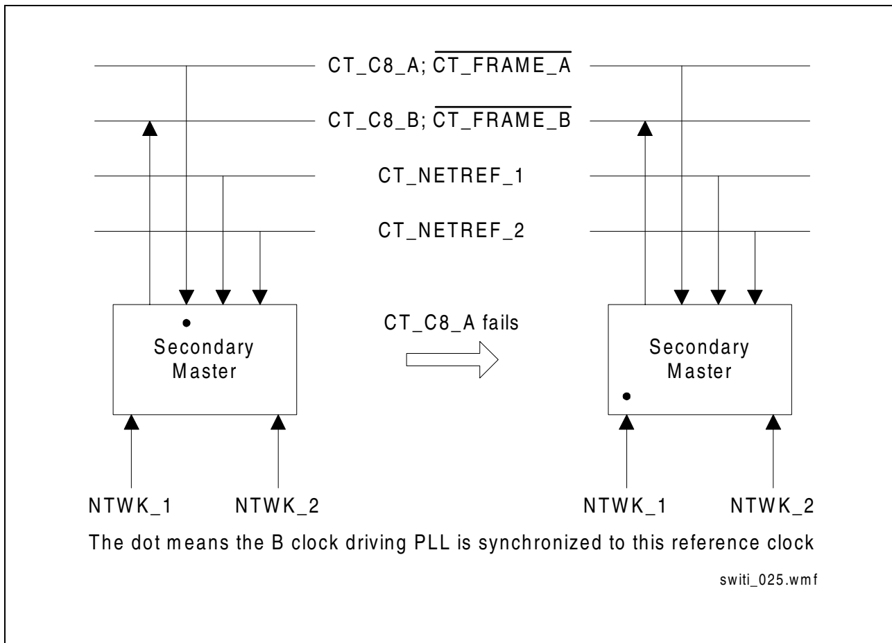
Figure 16 Clock Fallback of Secondary Master
