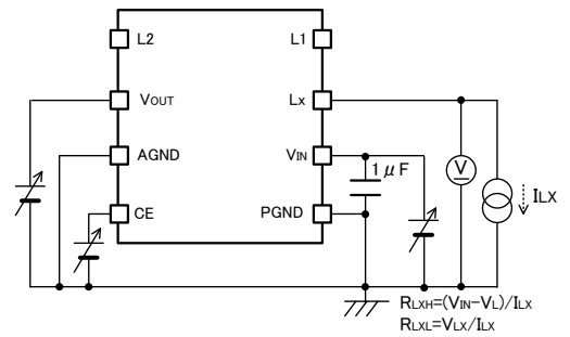
< Circuit No.⑥ >
