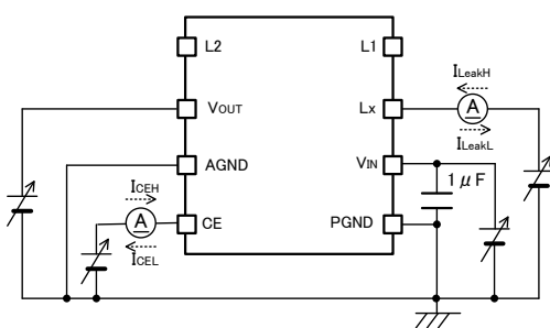
< Circuit No.⑦ >
