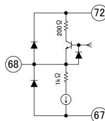
69: LOOP Filter
