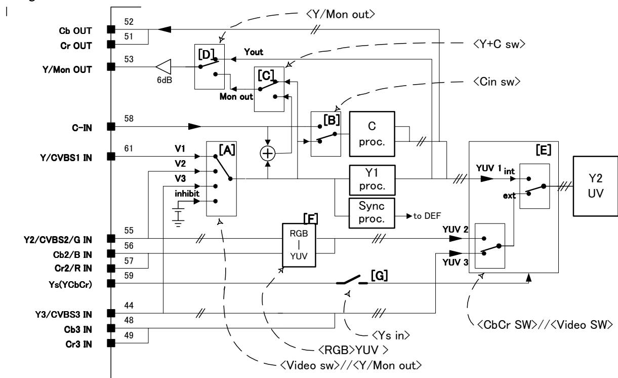
Fig. TB1261F Switch box
