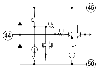
44: Y3/CVBS3 in
