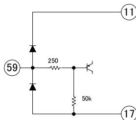
59: Ys (YCbCr)
