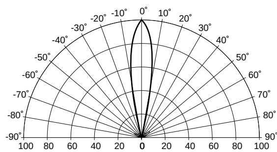
Fig. 4 Radiation Diagram
