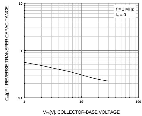
Figure 6. C_{re} - V_{CB}
