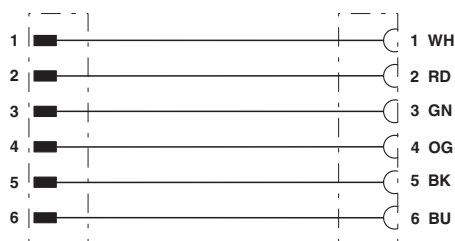
Contact assignment of 7/8" plugs/sockets
