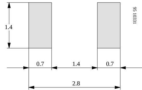
Figure 13. Recommended foot pads (in mm)
