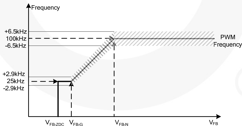
Figure 5. PWM Frequency
