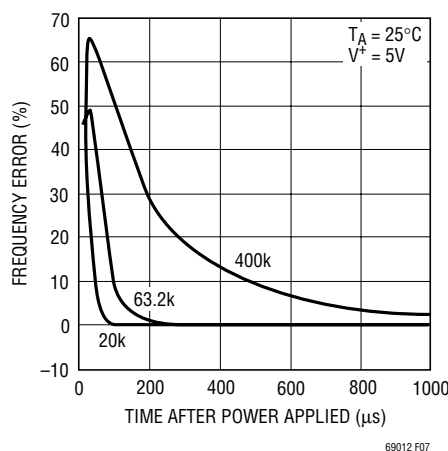
Figure 7. Start-Up Time
