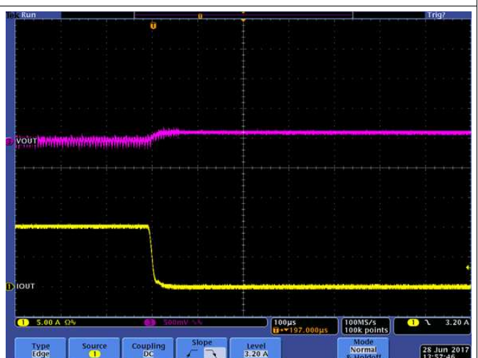
Transient Response
