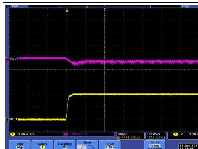
Transient Response
