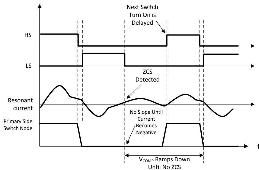
Figure 40. Timing Diagram of a ZCS Event
