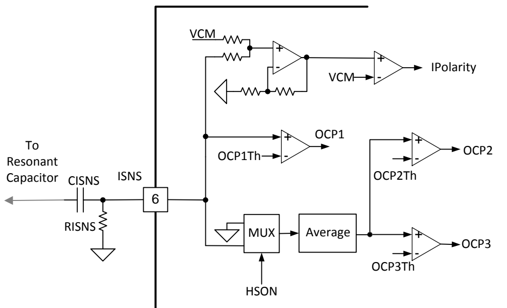
Figure 33. ISNS Block Diagram
