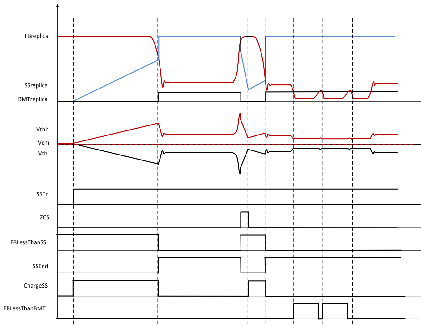
Figure 29. Feedback Chain Timing Diagram
