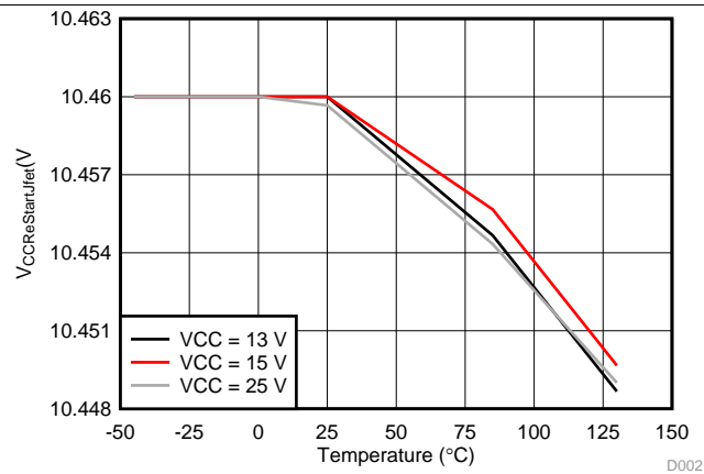
Figure 25. V_{CCReStartJfet} vs Temperature
