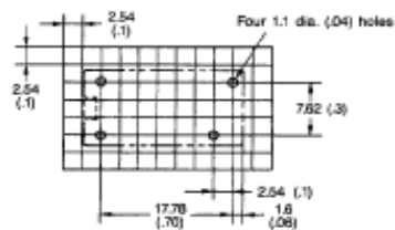
PC board dimensions (Bottom view)
