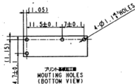
G5NB-E Footprint
