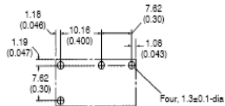
G5Q Footprint
