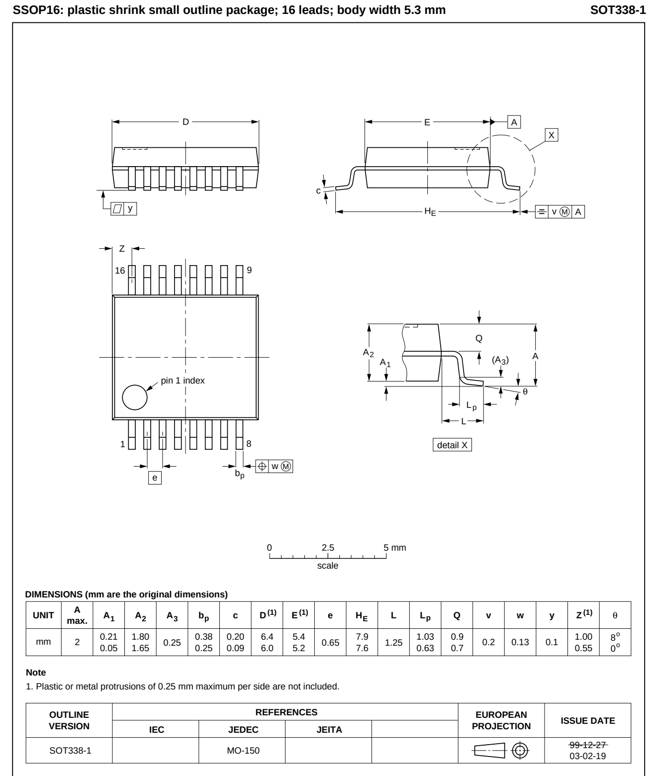
Fig 23. Package outline SOT338-1 (SSOP16)
