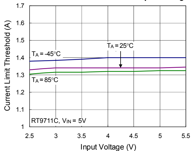
Current Limit Threshold vs. Input Voltage
