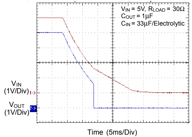
UVLO at Falling
