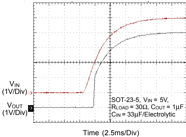
UVLO at Rising
