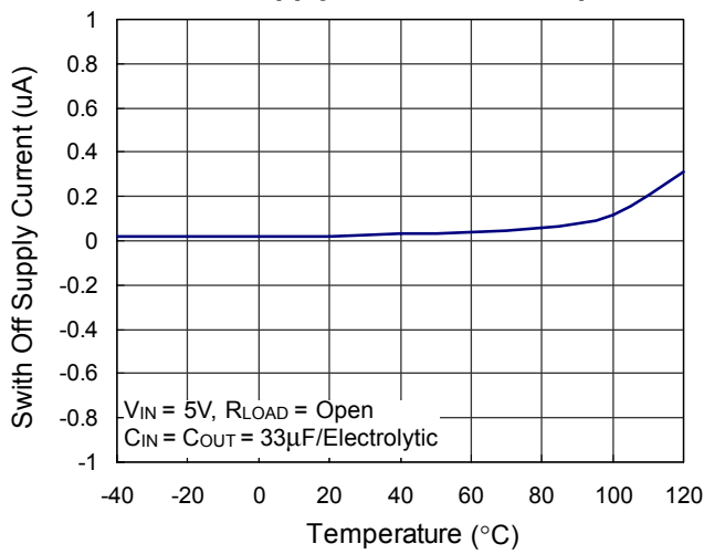
Swth Off Supply Current vs. Temperature
