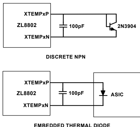
FIGURE 11. EXTERNAL TEMPERATURE MONITORING
