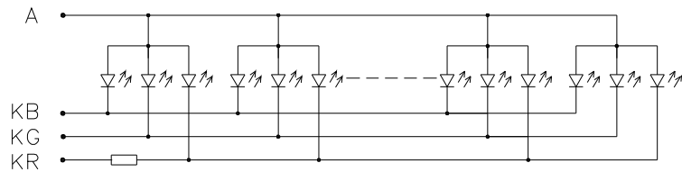
CIRCUIT DIAGRAM
