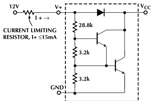
Figure 8. Shunt Regulator
