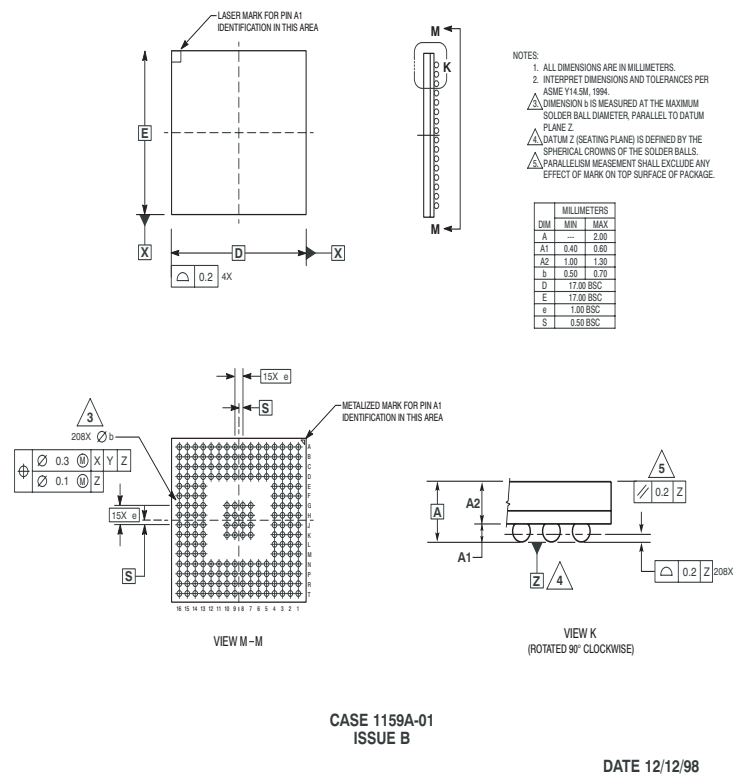
Figure B-1. 208MAPBGA Mechanical Dimensions
