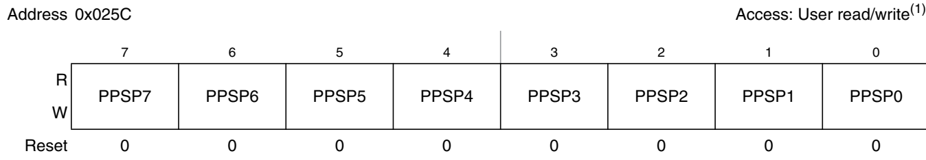
Figure 2-47. Port P Pull Device Enable Register (PERP)
