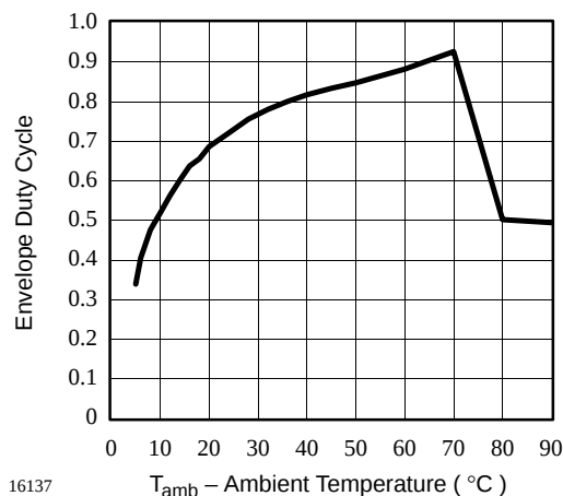
Figure 9. Envelope Duty Cycle vs. Ambient Temperature
