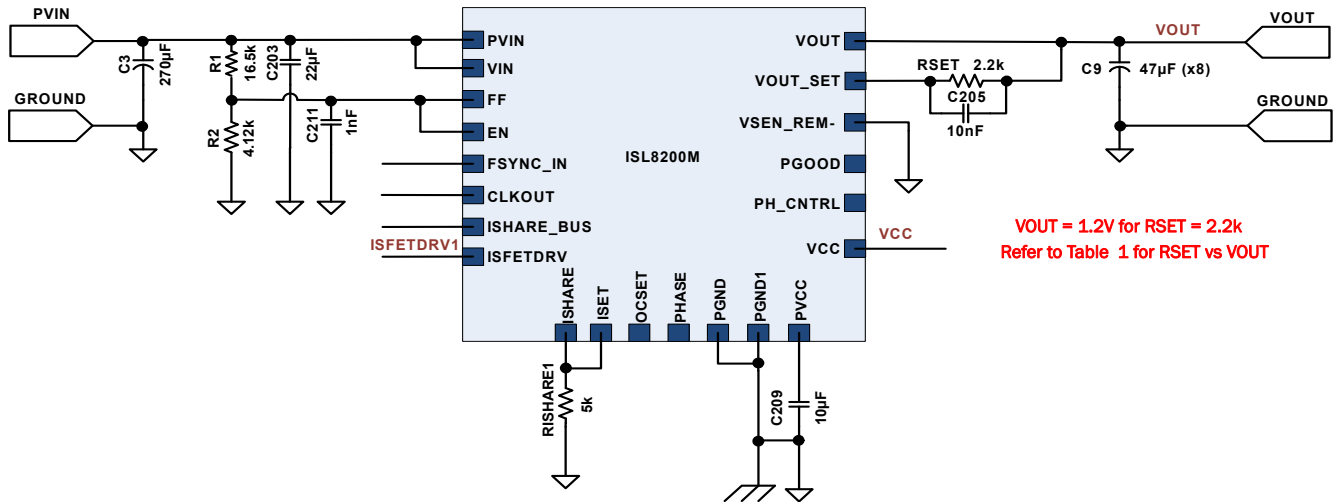
FIGURE 5. TEST CIRCUIT FOR ALL PERFORMANCE AND DERATING GRAPHS
