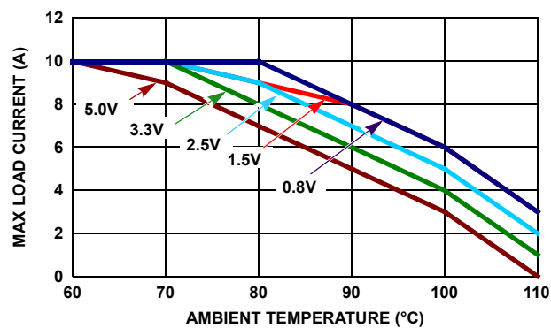
FIGURE 39. DERATING CURVE (12V IN ) 0 LFM FOR VARIOUS OUTPUT VOLTAGES
