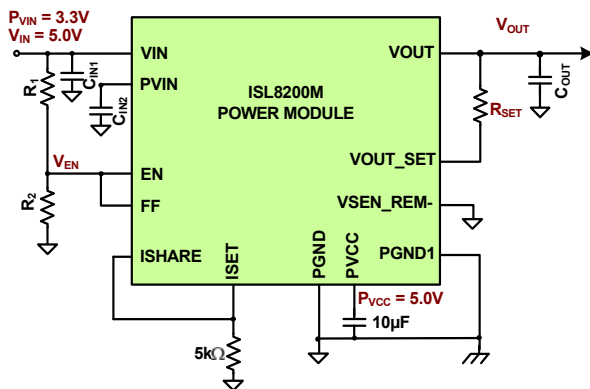
FIGURE 21. 3.3V OPERATION
