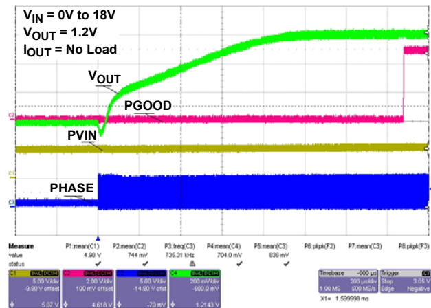
FIGURE 20. 50% PRE-BIAS START-UP
