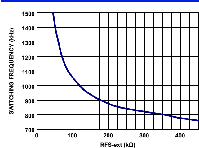
FIGURE 33. RFS-ext vs SWITCHING FREQUENCY
