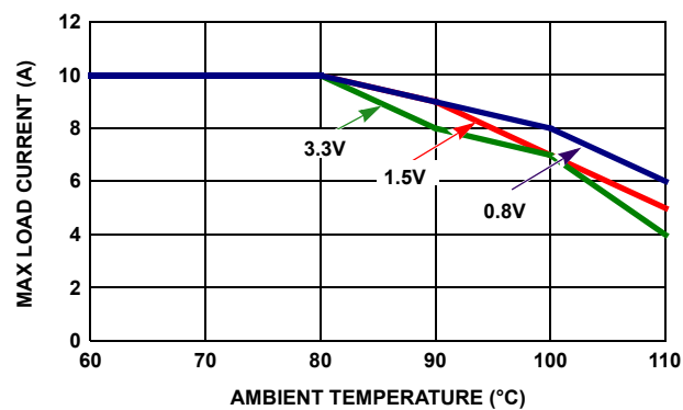
FIGURE 37. DERATING CURVE (5V IN ) 0 LFM FOR VARIOUS OUTPUT VOLTAGES
