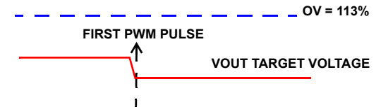
FIGURE 27. SOFT-START WITH V_{OUT} BELOW OV BUT ABOVE FINAL TARGET VOLTAGE
