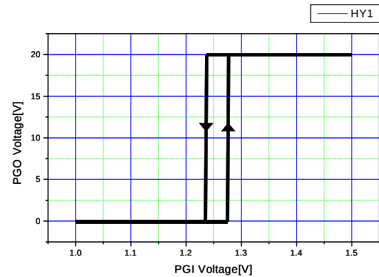
Figure 11. Hysteresis Voltage 1
