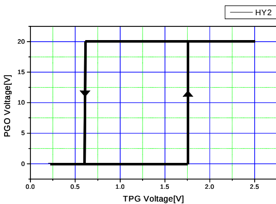
Figure 12. Hysteresis Voltage 2
