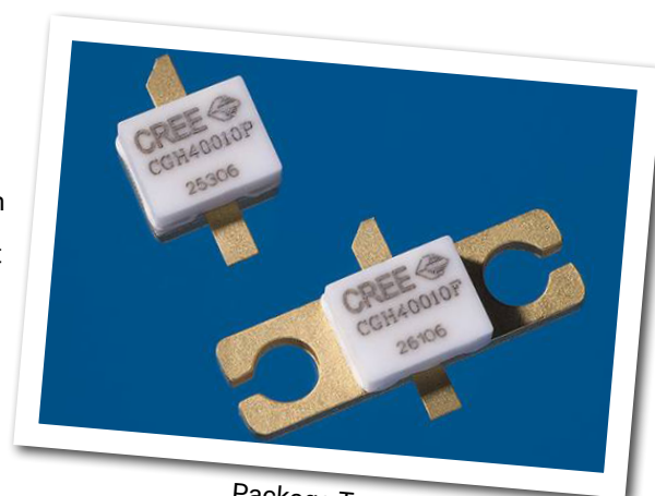
Package Types: 440166, & 440196 PN's: CGH40010F & CGH40010P
