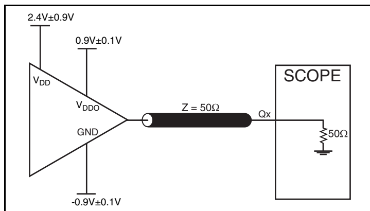
3.31.8V Core/1.8V LVCMOS Output Load AC Test Circuit
