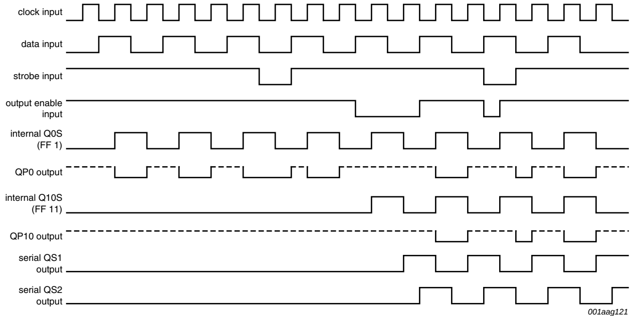
Fig 5. Timing diagram
