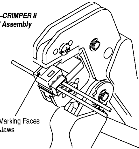
AMP Hand Tool 231839-1
