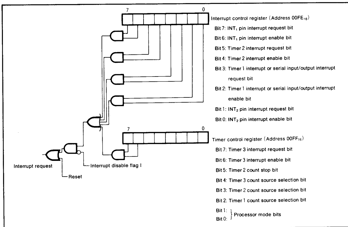
Fig.3 Interrupt control
