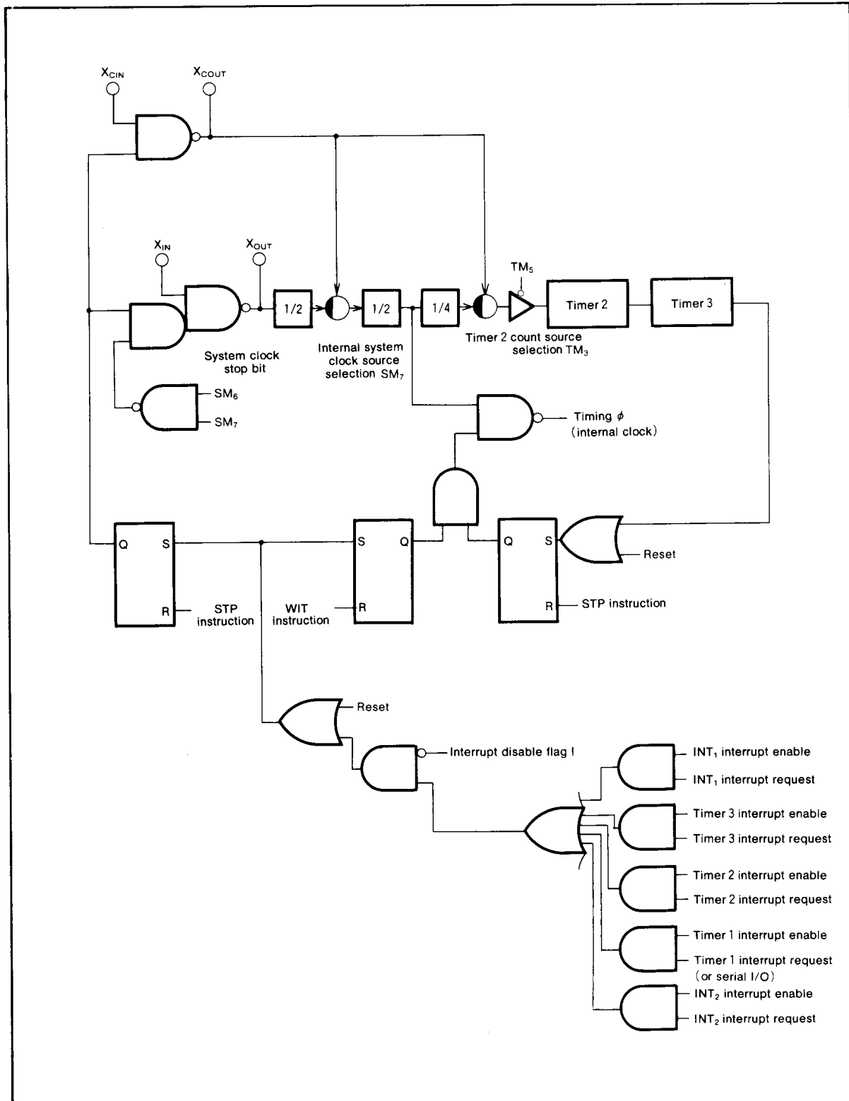
Fig.26 Block diagram of clock generating circuit
