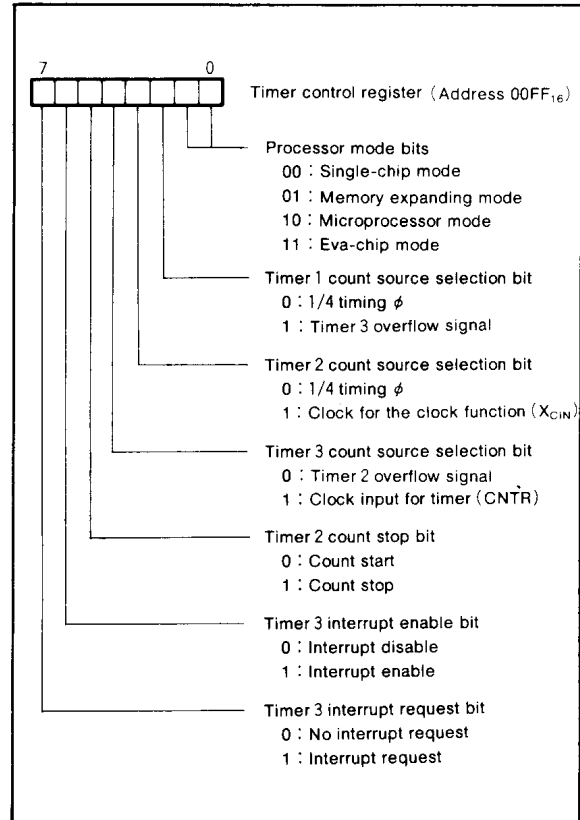
Fig.4 Structure of timer control register
