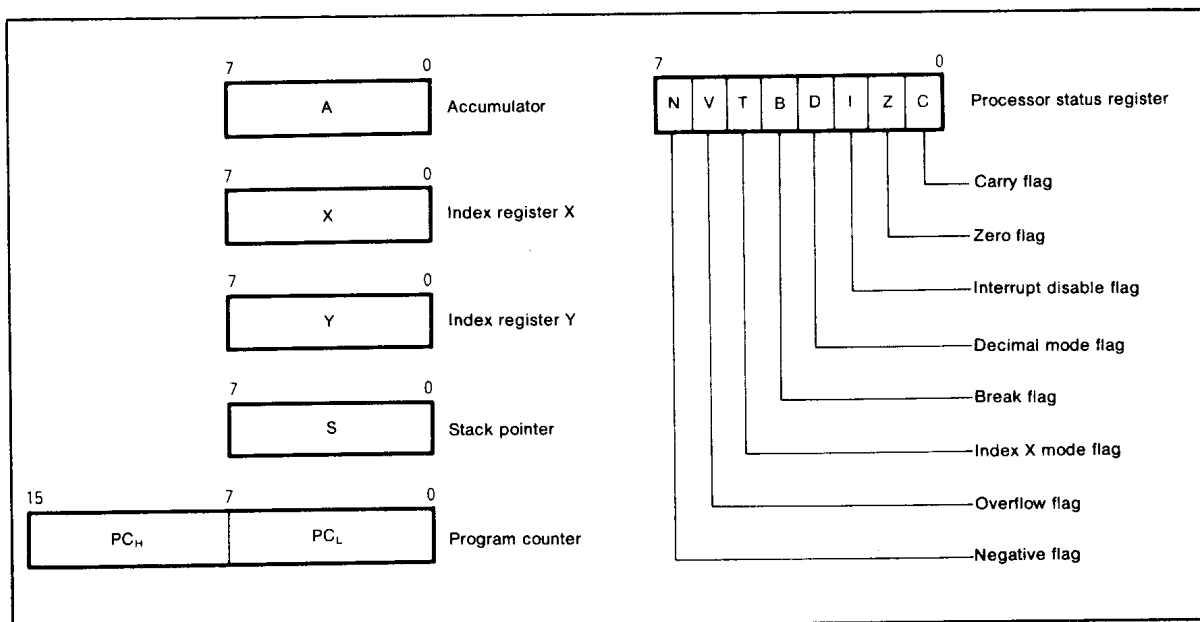
Fig.2 Register structure
