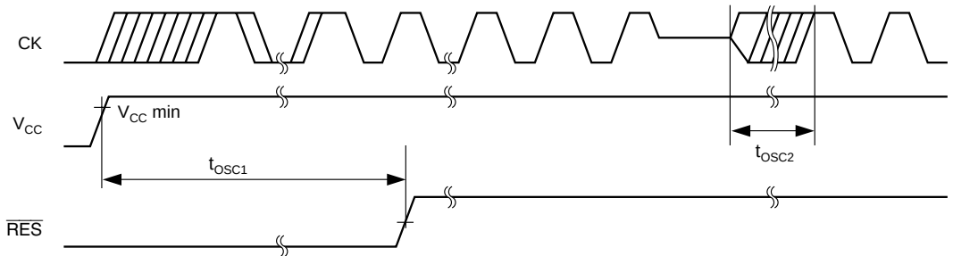
Figure 25.3 Oscillation Settling Time
