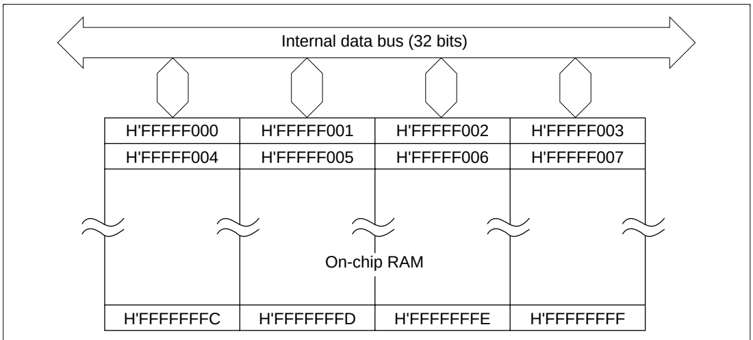
Figure 23.1 Block Diagram of RAM
