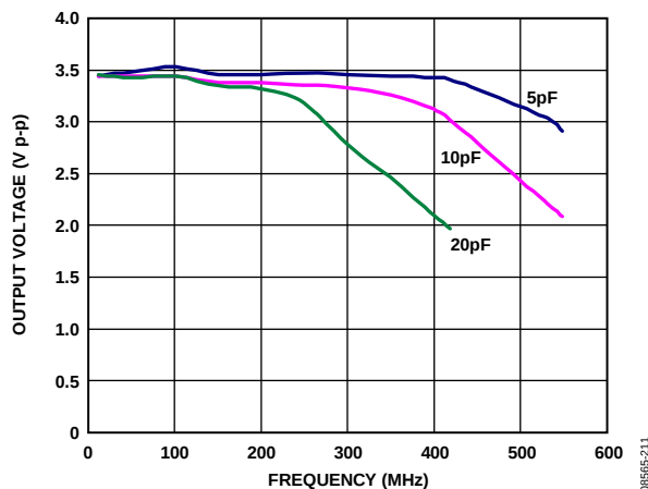
Figure 17. Peak-to-Peak Output Voltage vs. Frequency, CMOS
