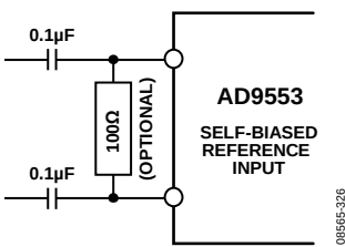
Figure 26. Reference Input
