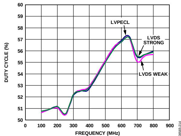
Figure 20. Duty Cycle vs. Output Frequency, LVPECL and LVDS (100 Ω Load)
