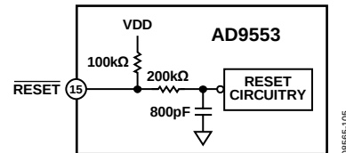
Figure 33. Power-On Reset
