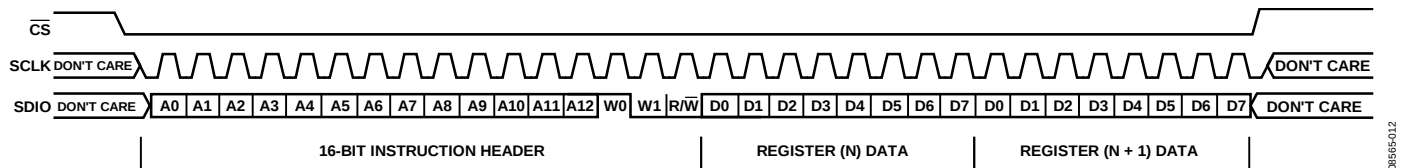
Figure 40. Serial Control Port Write—LSB First, 16-Bit Instruction, Two Bytes Data
