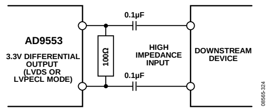
Figure 24. AC-Coupled LVDS or LVPECL Output Driver
