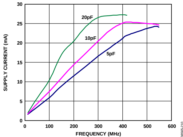
Figure 16. Supply Current vs. Output Frequency, CMOS (10 pF Load)
