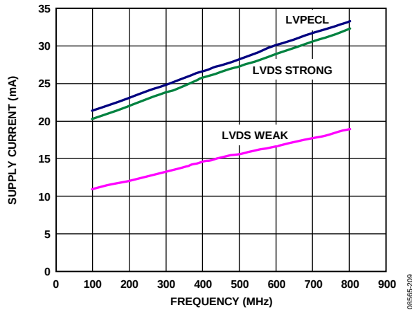
Figure 15. Supply Current vs. Output Frequency, LVPECL and LVDS (10 pF Load)
