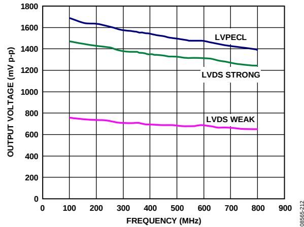
Figure 18. Peak-to-Peak Output Voltage vs. Frequency, LVPECL and LVDS (100 Ω Load)
