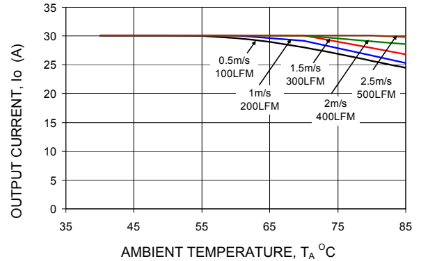
Figure 34. Derating Output Current versus Ambient Temperature and Airflow (ATH030A0X3-SRH).
