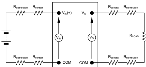
Figure 44. Output Ripple and Noise Test Setup.
