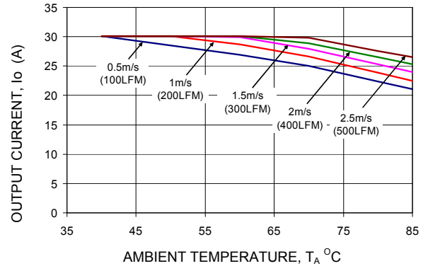
Figure 13. Output Current Derating versus Ambient Temperature and Airflow (ATS030A0X3-SRH).
