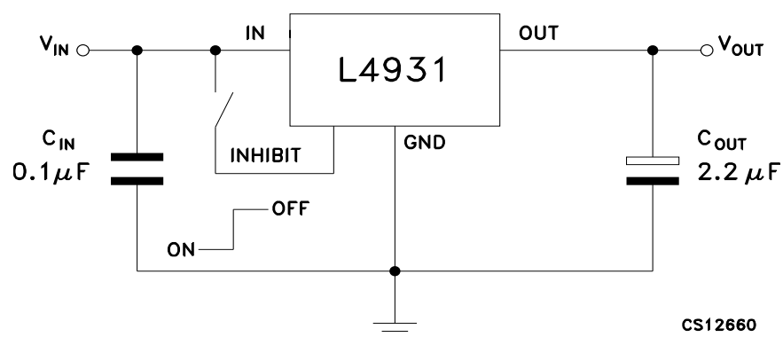
Figure 3. Test circuit
