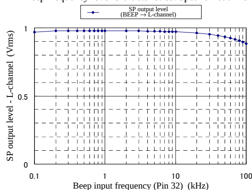
Beep frequency level characteristics: Speaker load – 8\ \Omega
