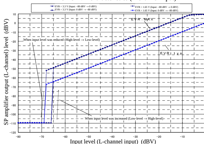
SP-SAVE characteristics (L-channel input)
