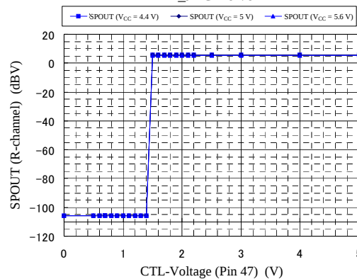
HP_JACK on/off
