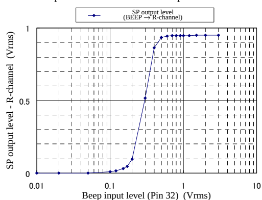
Beep I/O level characteristics: Speaker load – 8\ \Omega
