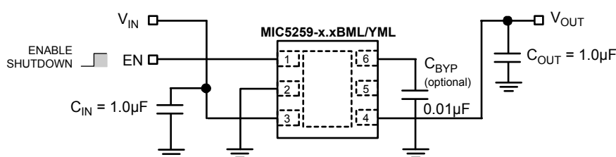
Ultra-Low Noise Regulator Application
