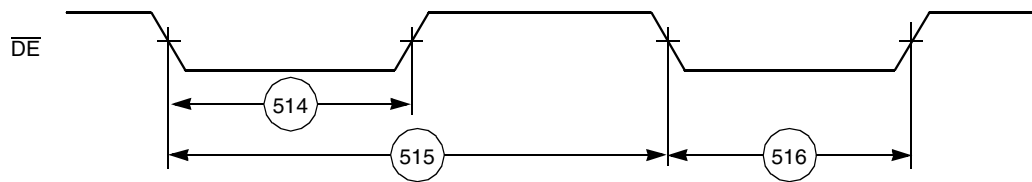
Figure 2-32. OnCE—Debug Request
