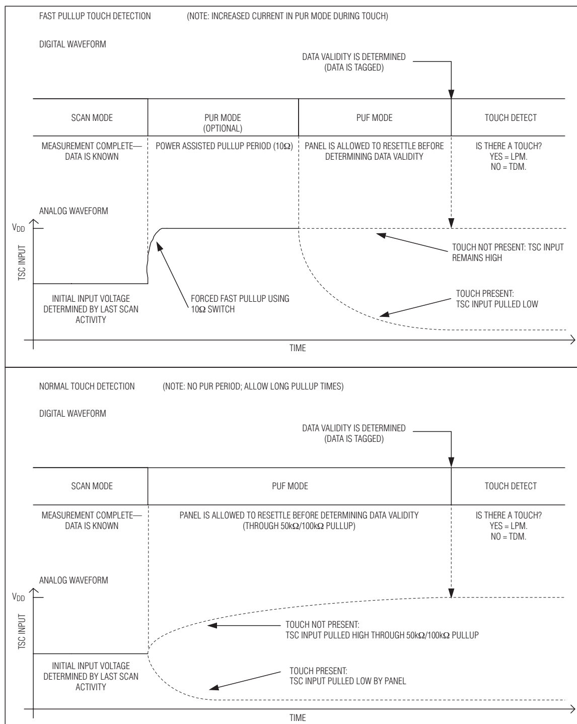
Figure 7. Touch-Detection Operations
