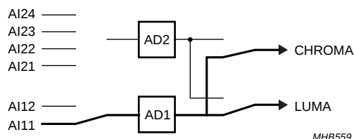
Fig.43 Mode 0; CVBS (automatic gain).
