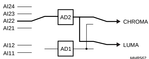
Fig.46 Mode 3; CVBS (automatic gain).
