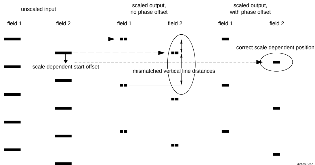
Fig.28 Basic problem of interlaced vertical scaling (example: down-scale \frac{3}{5} ).
