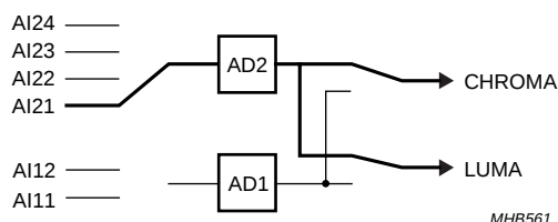
Fig.45 Mode 2; CVBS (automatic gain).
