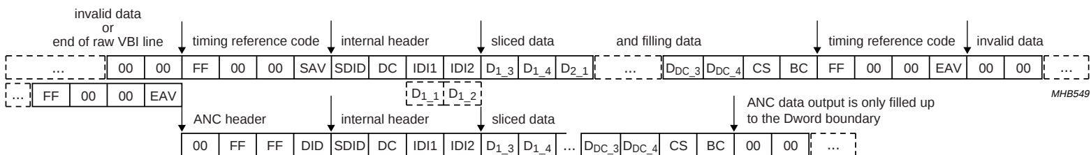
Fig.30 Sliced data formats on the I-port in 8-bit mode.
