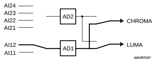
Fig.44 Mode 1; CVBS (automatic gain).
