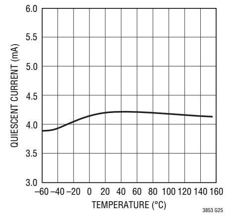
Quiescent Current vs Temperature Without EXTV CC
