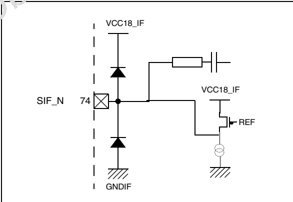
Figure 36. VCC18_IF
