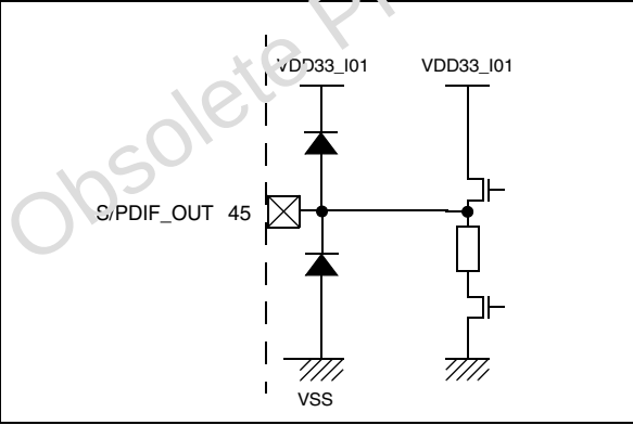
Figure 41. S/PDIF_OUT
