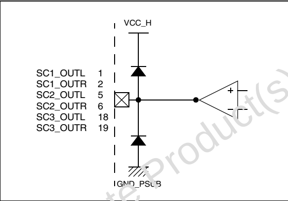
Figure 33. SC_OUT
