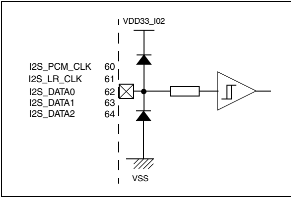
Figure 44. I 2 S
