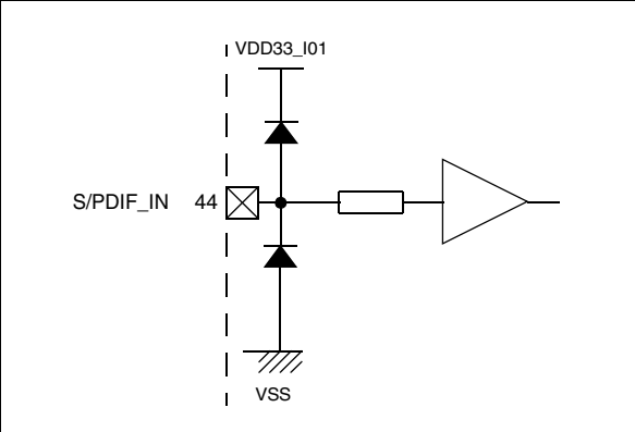
Figure 43. S/PDIF_IN
