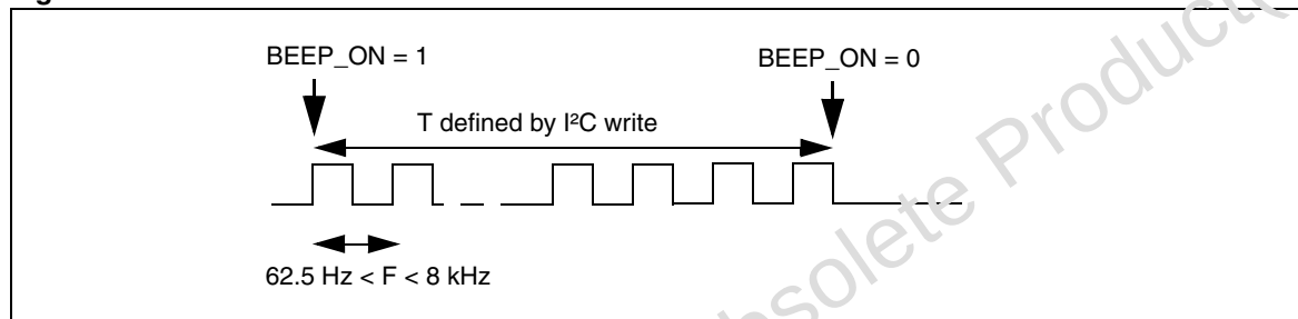
Figure 18. Continuous mode
