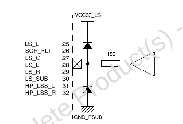
Figure 34. VCC33_LS
