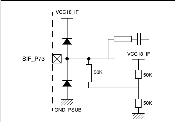
Figure 32. SIF_P
