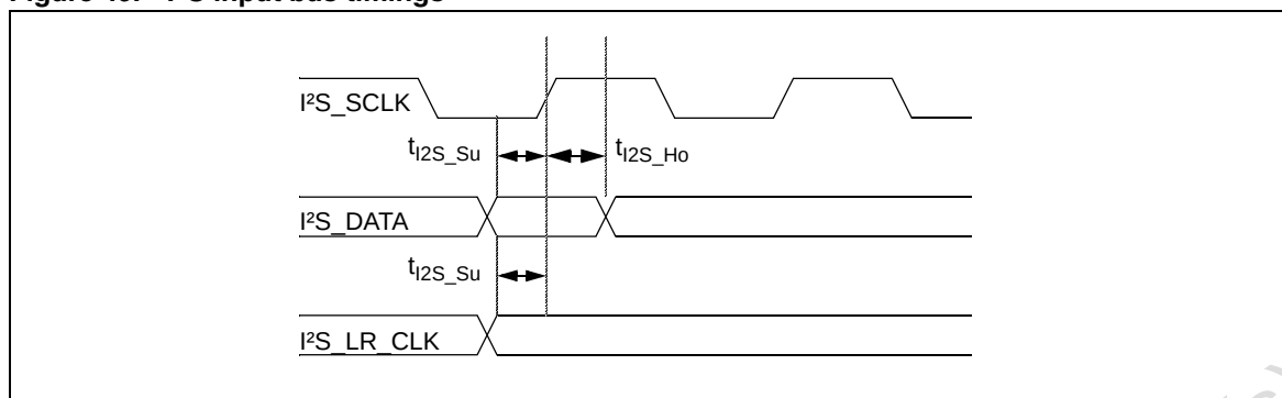
Figure 49. I 2 S input bus timings
