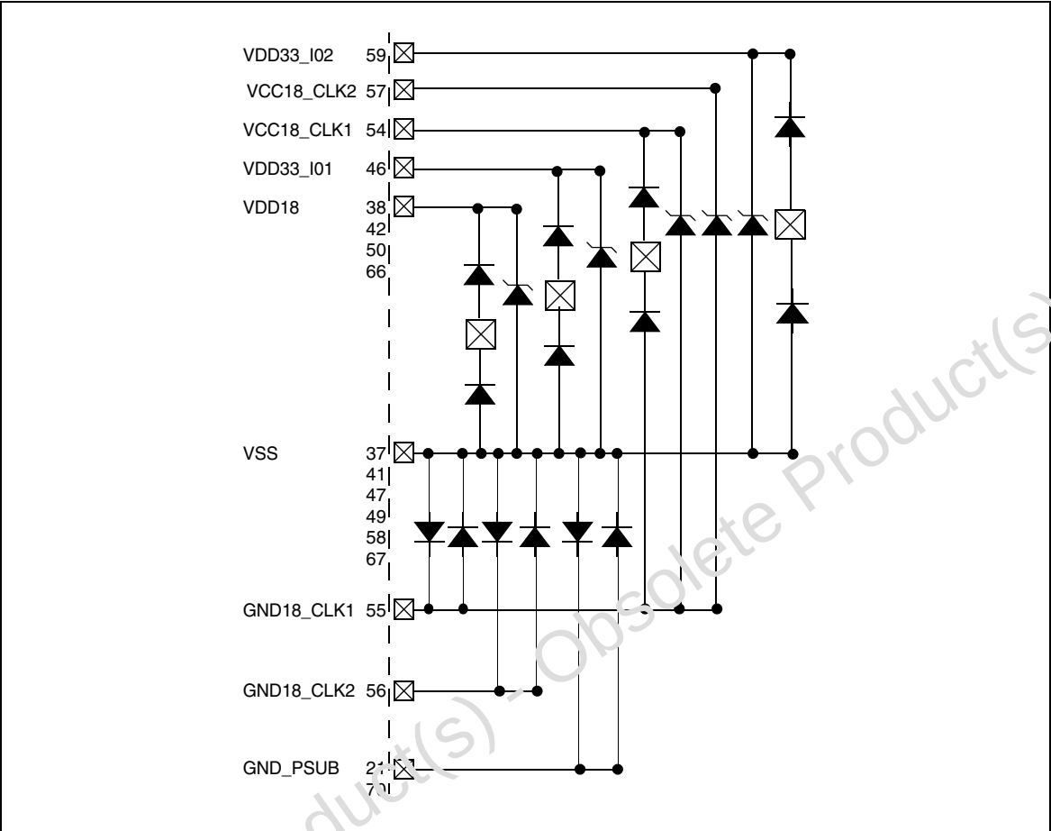
Figure 48. VSS
