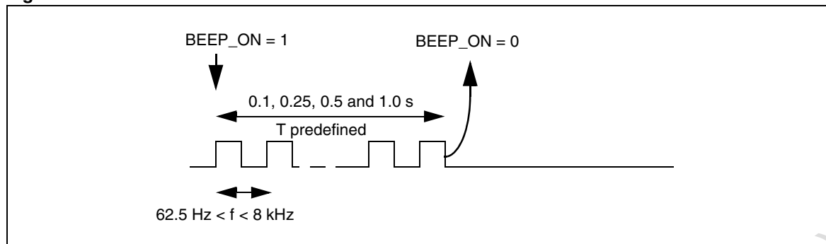
Figure 17. Pulse mode
