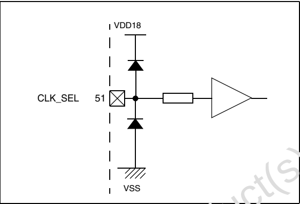
Figure 45. CLK_SEL
