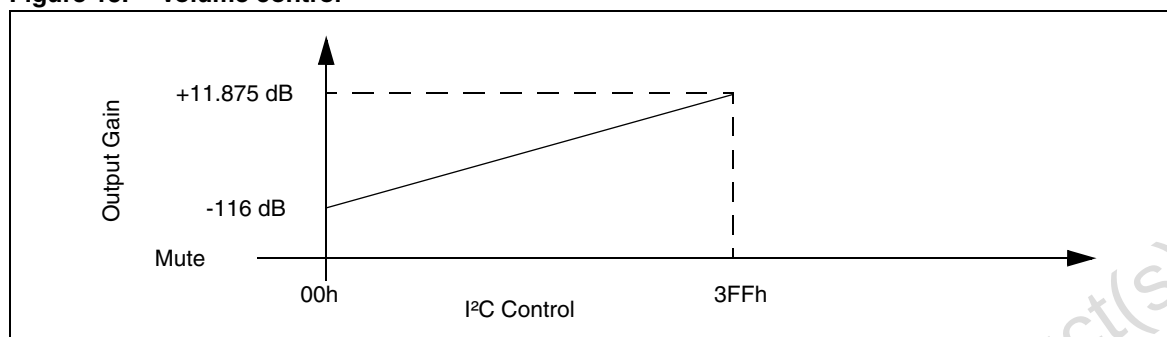
Figure 15. Volume control
