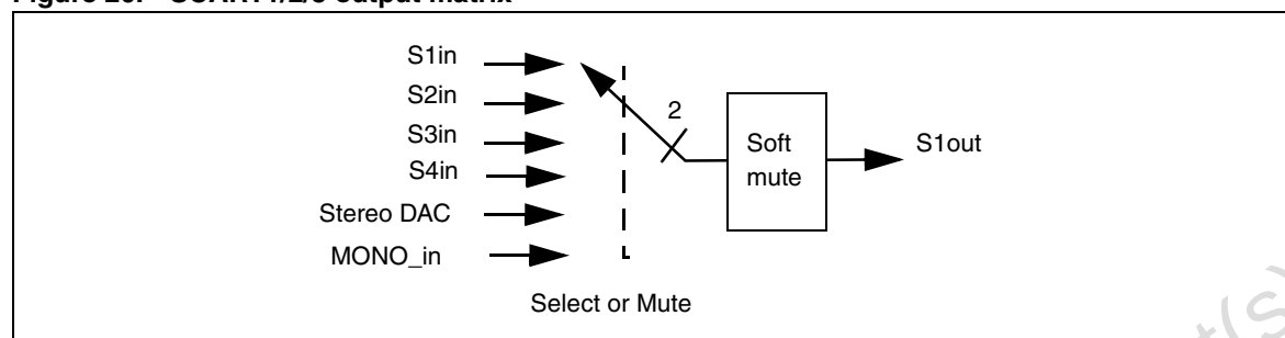
Figure 20. SCART1/2/3 output matrix
