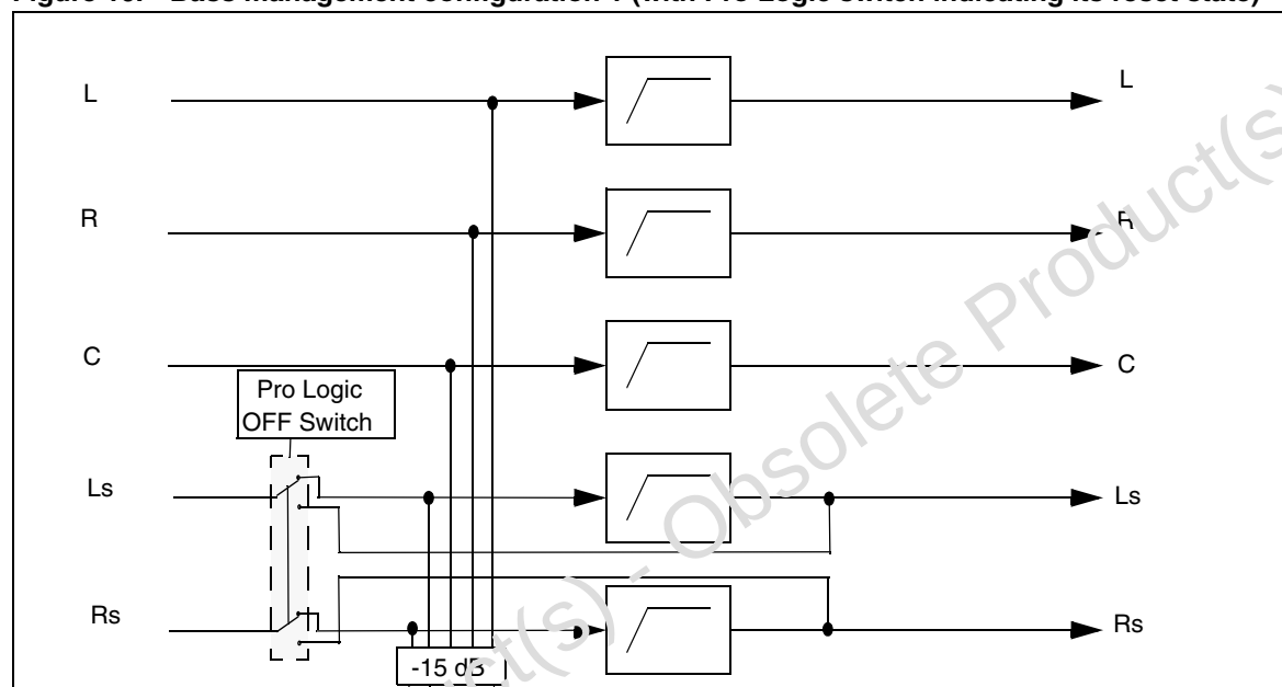
Figure 10. Bass management configuration 1 (with Pro Logic switch indicating its reset state)
