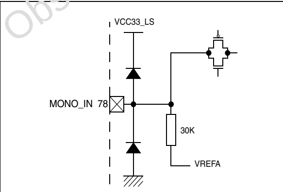
Figure 35. MONO_IN
