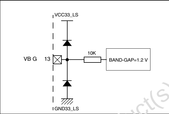
Figure 39. VBG
