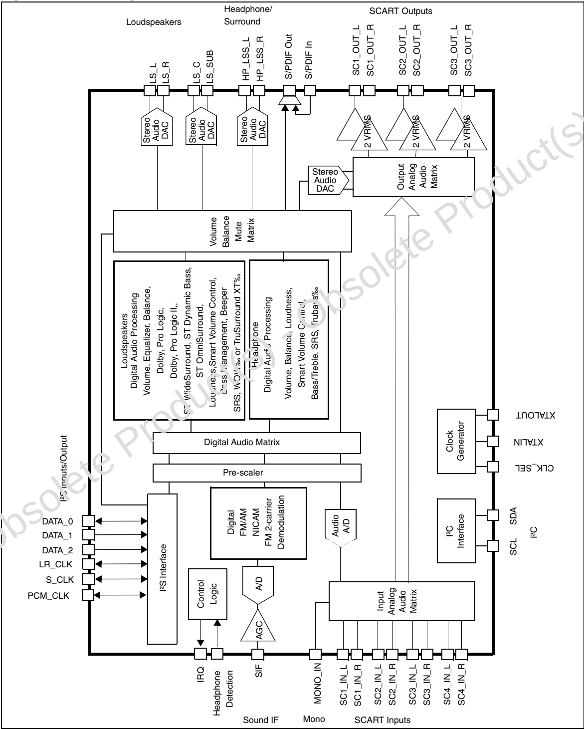
Figure 5. Block diagram
