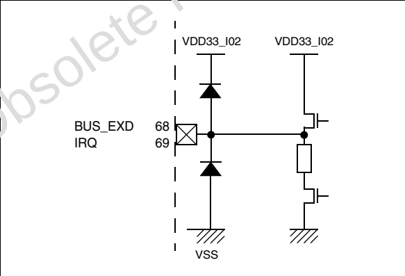
Figure 42. BUS_EXD_IRQ
