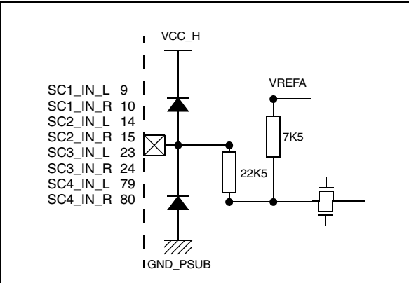
Figure 37. SC_IN
